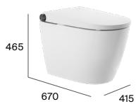
In-Wash® Gap cold water Round 305 DC A80349C00V
